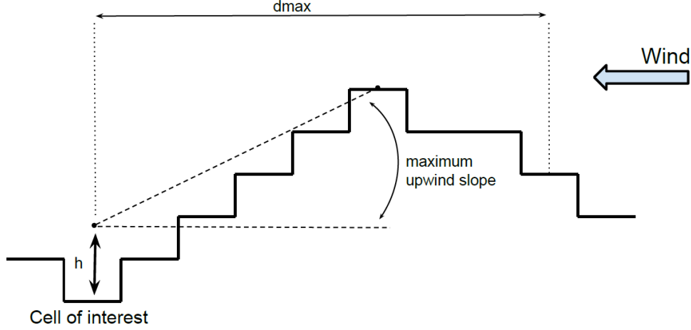
Figure 11: Schematic view of the up-wind slope Sx . From the cell of interest, the upwind cells of the DEM are investigated until a defined distance d_{max} to find the cell that has the greatest slope.
