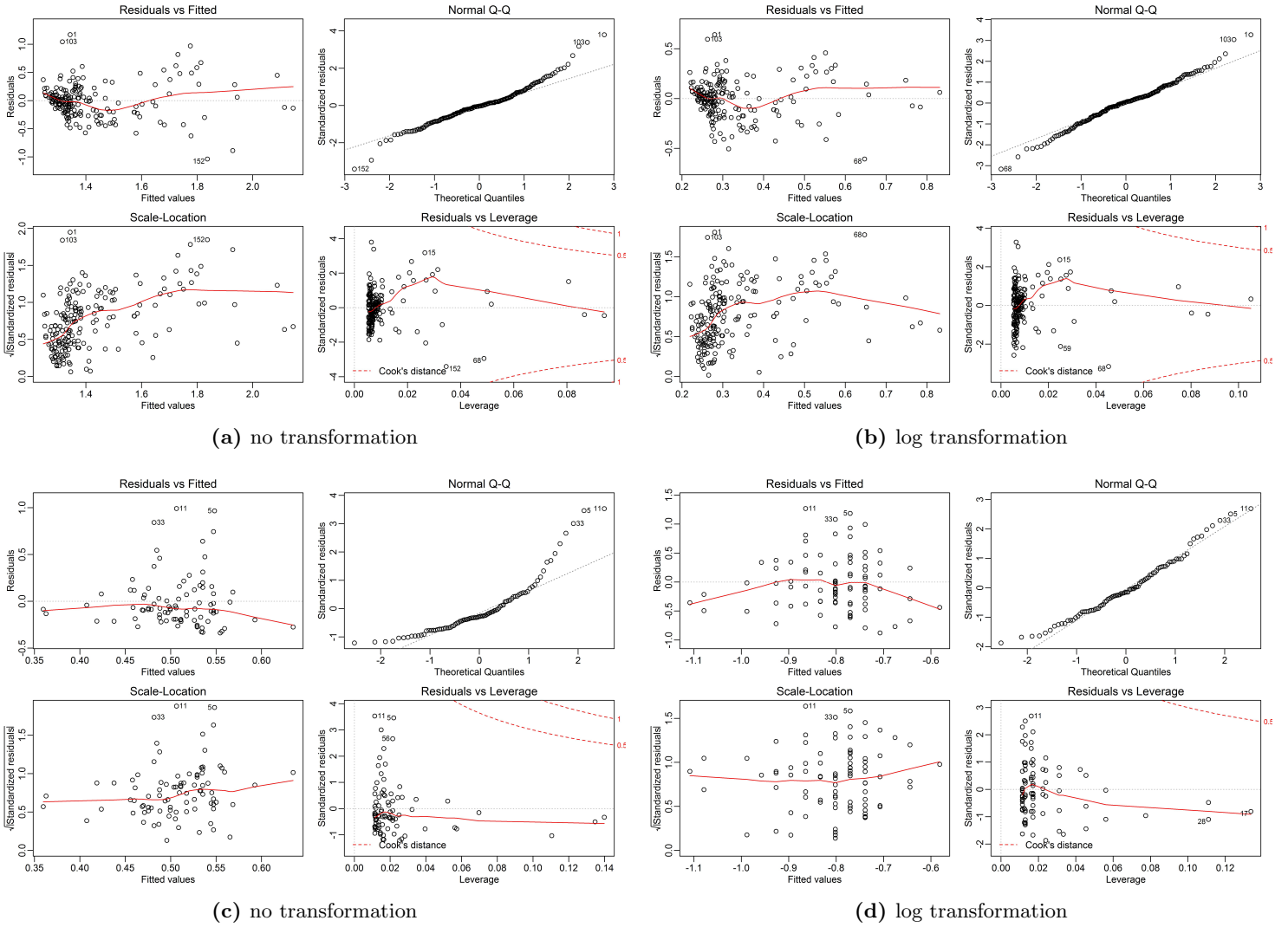
Figure 68: Diagnostic plot of the linear models built in Longyearbreen and SFS for the 50m DEM.
