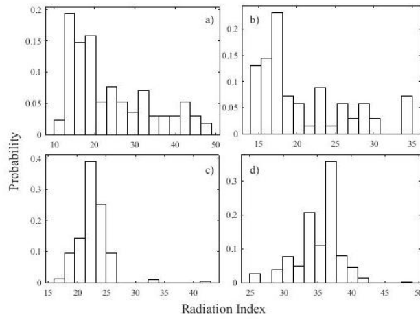
Figure 63: Distribution of samples radiation index values in a) Breinosa, b) Larsbreen, c) Longyearbreen and d) South Facing Slope.
