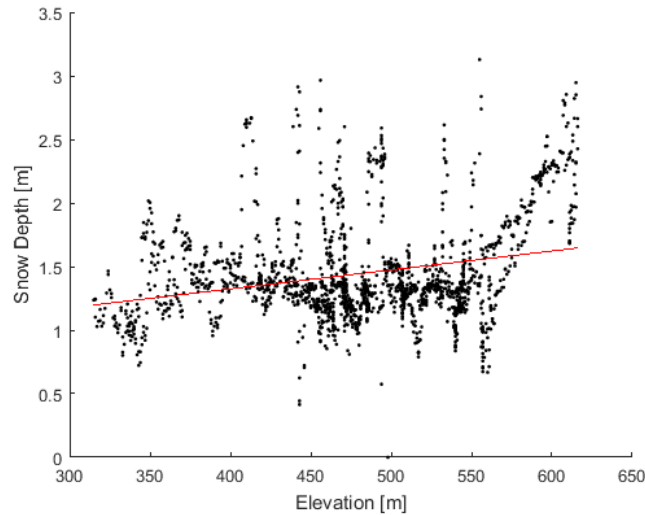
Figure 40: Linear regression to obtain the elevation gradient model in site 3 for 5 m resolution. The regression confirms that there is a positive correlation between elevation and snow depth.
