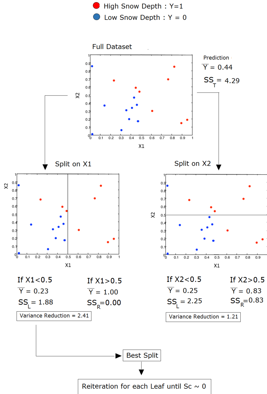
Figure 14: Example of regression tree algorithm working on two predictors, X_1 and X_2 , of the dependent variable snow depth. Starting from a root, i.e. the full dataset, the algorithm estimates the first optimal split for each of the two predictors. In this case there are two possibilities : split on X_1 or split on X_2 . Splitting the dataset creates two new subsets, also called leaves or snow classes. The mean value of a leaf is the prediction of the regression tree for the specific sequence of predictors' values that leads from the root to the leaf. In each snow class the variability of the data is evaluated according to equation 8. Eventually the total reduction in variability given by the split is evaluated and compared to the one achieved by splitting the root on a different predictor. The best split is the one that achieves the maximum reduction in variability, in this case the split on X_1 . The process is reiterated treating each leaf as a root until the total reduction in variance approaches the null value.
