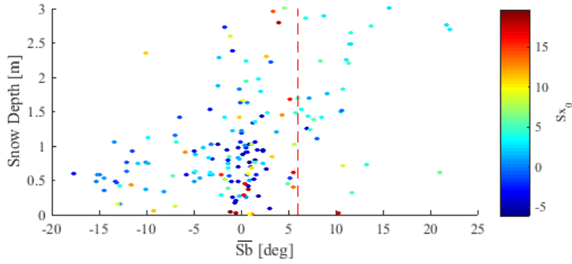
Figure 20: Scatter plot indicating snow depth versus \overline{S_b} . The scatter is graduated with S_{x_0} . Blue points that have also high \overline{S_b} represent locations that are located in the influence zone of a slope break exposed to wind. They are therefore more likely to be subjected to enhanced snow accumulation.
