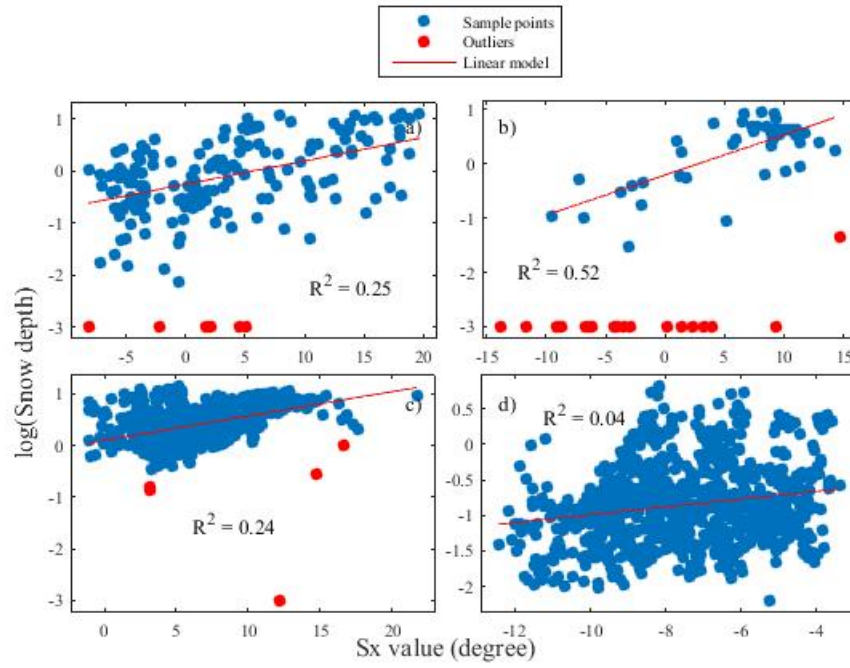
Figure 70: Calibration result of precipitation Sx in a) Breinosa, b) Larsbreen, c) Longyearbreen and d) South Facing Slope. In Larsbreen the Sx used is the one calculated with the optimal h and dmax found in Longyearbreen. The outliers that have a \log(\text{snow depth}) of -3 are the samples where measured snow depth was zero and this value was manually given to them so that they appear on the plot.
