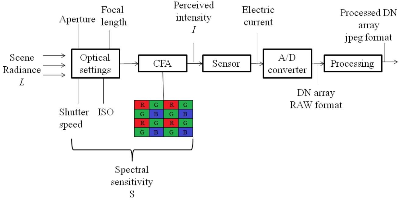
Figure 43: Schematic view of a digital camera.
